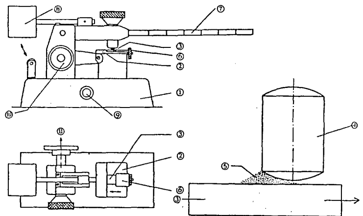
Fig. 14: Friction apparatus; elevation and plan view
