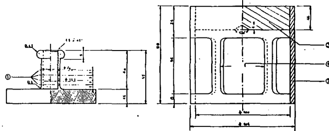
Fig. 17: Bell-shaped mass of 2 220 g capable of being suspended on the bronze piston
