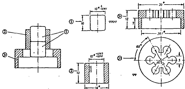
Fig. 12: Impact device for substances in powdered or paste-like form dimensions in mm
