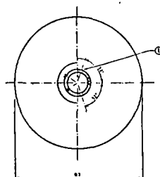
Fig. 16: Hollow bronze cylinder. closed at one end; plan and vertical section
