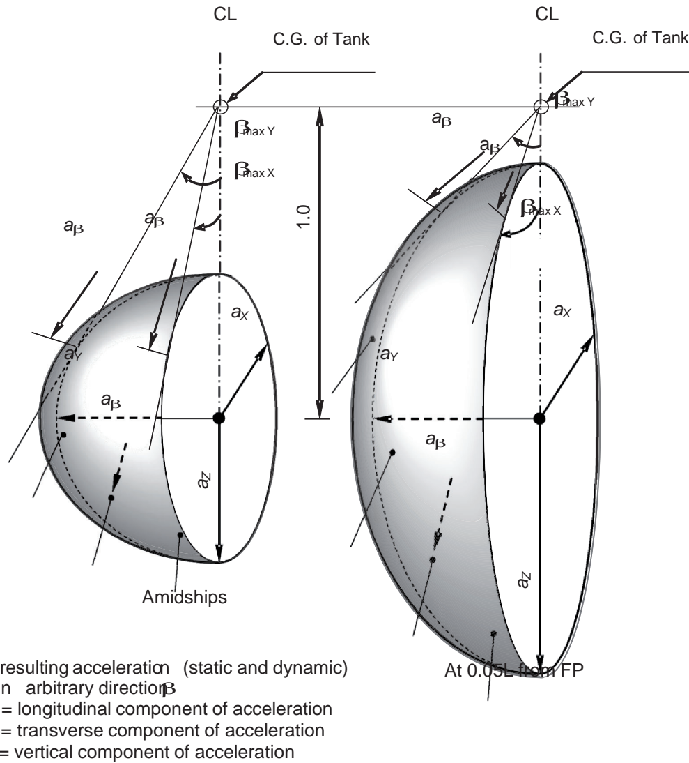
Figure 4.1 – Acceleration ellipsoid
