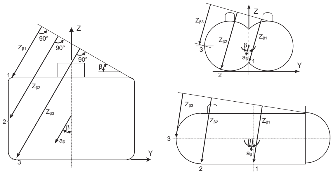
Figure 4.2 – Determination of internal pressure heads
