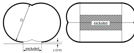
Bilobe tanks
