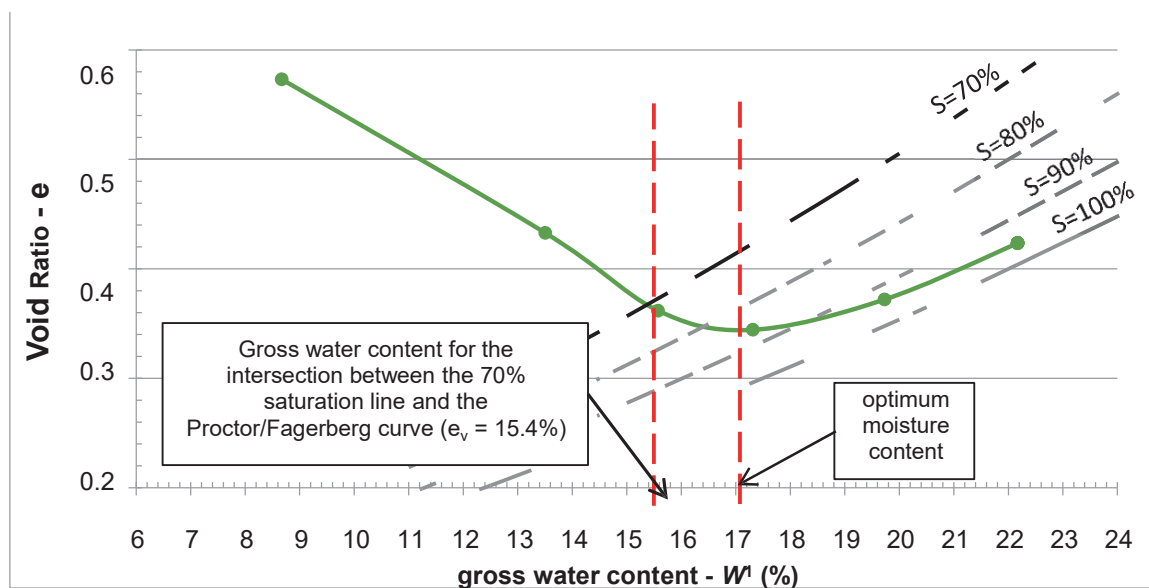
Figure 1.5.5.3.7 – Example of a measured compaction curve for void ratio versus gross water content with the 70%, 80%, 90% and 100% degree of saturation lines plotted
