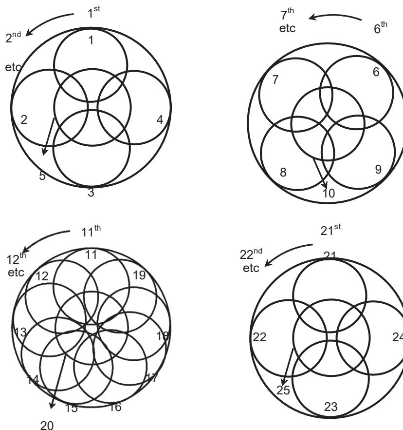
Figure 1.5.5.3.2 – Recommended compaction patterns
