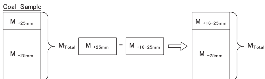
Figure 1.5.5.2.2.2 – Overview of sample reconstitution (Method 2)
