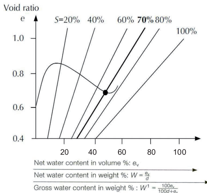
Figure 1.5.5.3.6 – Typical compaction curve
