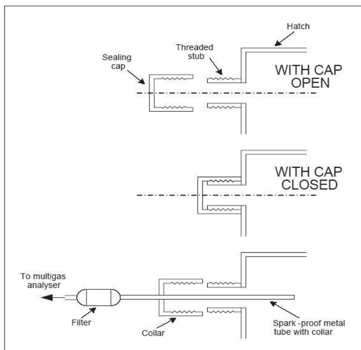
Diagram of gas sampling point
