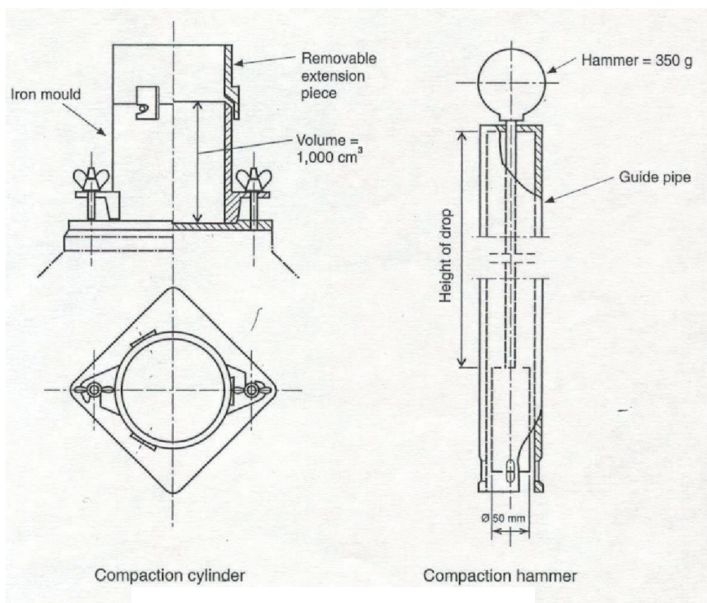
Figure 1.3.2 – Proctor apparatus
