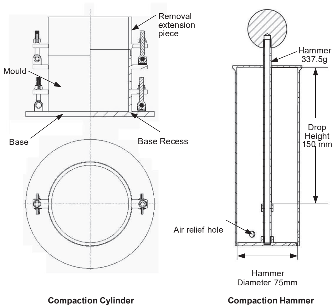
Figure 1.5.5.1.3.2 – Schematic of a Proctor/Fagerberg apparatus
